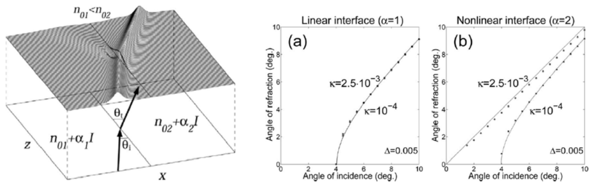
Figure 1. (Left) Typical interface geometry and (right) predictions of soliton refraction using the new Snell law, \gamma n_{01} \cos \theta_i = n_{02} \cos \theta_r , where \gamma is a universal function of system and beam parameters.
